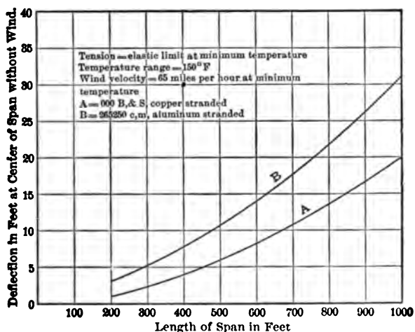
FIG. 3. DEFLECTION CURVE AT MAXIMUM TEMPERATURE.
